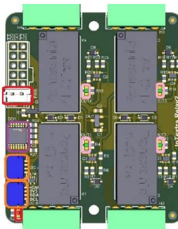
PWR and Qwiic®
